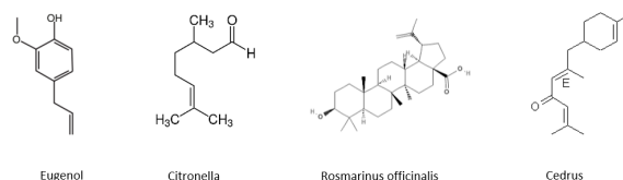
Figure 1: Chemical structures of essential oil
