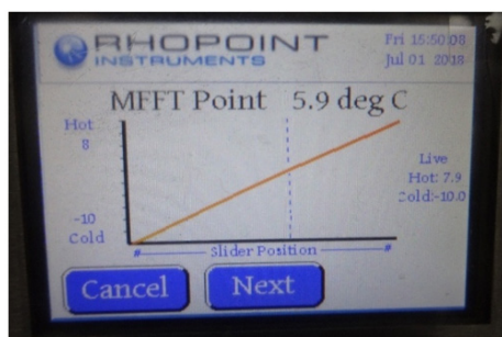
Figure 11: MFFT temperature
